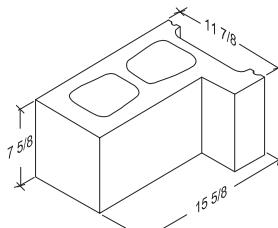
12-8-16 L-Corner 11 3/8" x 7 3/8" x 15 5/8"
