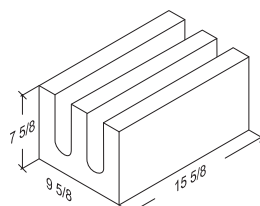
10-8-16 CBBB 9 5/8" x 7 5/8" x 15 5/8"
