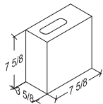
4-8-8 Half 3 3/8" x 7 3/8" x 7 5/8"
