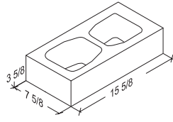
8-4-16 Half High 7 5/8" x 3 5/8" x 15 5/8"
