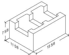
12-8-16 Bond Beam 11 3/8" x 7 3/8" x 15 5/8"
