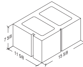
12-8-16 1-Score 11 3/8" x 7 3/8" x 15 5/8"
