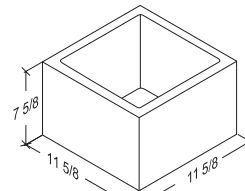
12 x 8 x 12 Pilaster 11 3/8" x 7 3/8" x 11 3/8"
