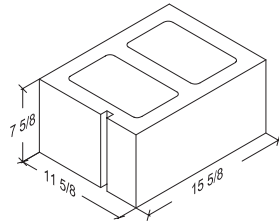
12-8-16 Square Corner 11 3/8" x 7 3/8" x 15 5/8"
