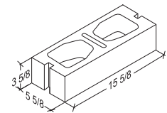
6-4-16 Half High Partition 5 5/8" x 3 3/8" x 15 5/8"
