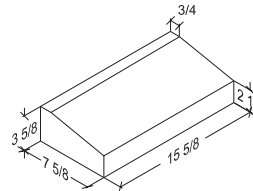
8 x 4 x 16 Slope Sill 9 3/8" x 3 3/8" x 15 5/8"
