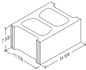
12-8-16 Standard 11 3/8" x 7 3/8" x 15 5/8"
