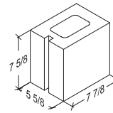
6-8-8 Half 5 5/8" x 7 3/8" x 7 7/8"
