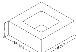
17 x 7 x 17 Chimney Block 16 3/4" x 7" x 16 3/4"
