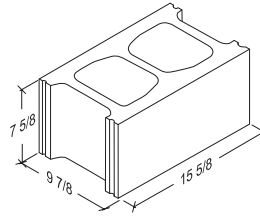
10-8-16 Standard 9 5/8" x 7 5/8" x 15 5/8"
