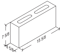
4-8-16 3 3/8" x 7 3/8" x 15 5/8"
