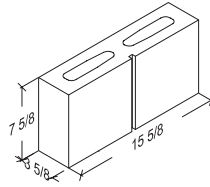
4-8-16 1-Score 3 3/8" x 7 3/8" x 15 5/8"
