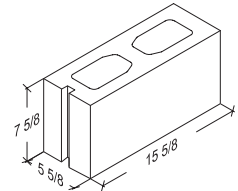
6-8-16 Square Corner 5 5/8" x 7 3/8" x 15 5/8"
