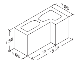
6 Inch L-Corner 7 3/8" x 7 3/8" x 15 5/8"
