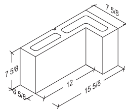
4 Inch L-Corner 7 3/8" x 7 3/8" x 15 5/8"
