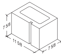
12-8-8 Half 11 3/8" x 7 3/8" x 7 3/8"
