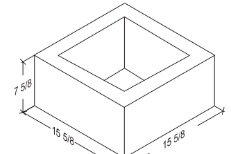
16 x 8 x 16 Chimney Block 15 3/8" x 7 3/8" x 15 5/8"
